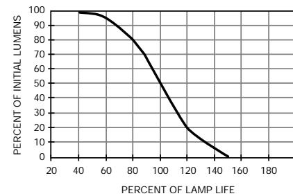
Typical Mortality Curve for Incandescent Lamps
