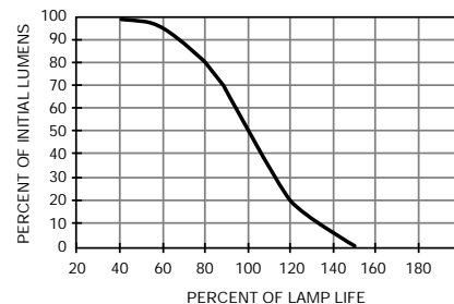
Typical Mortality Curve for Incandescent Lamps
