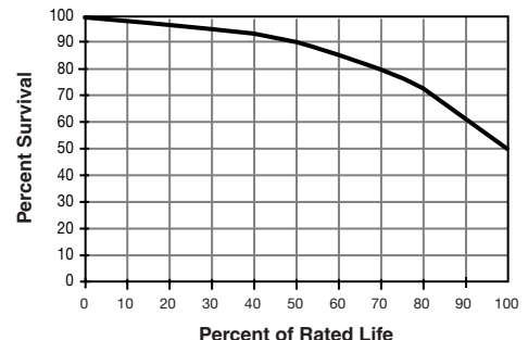
Typical Survival Curve (1000W)
