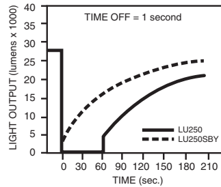
Lumen Output vs. Time
