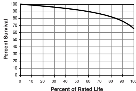
Typical Survival Curve (70, 100, 150, 200, 250, 400W)
